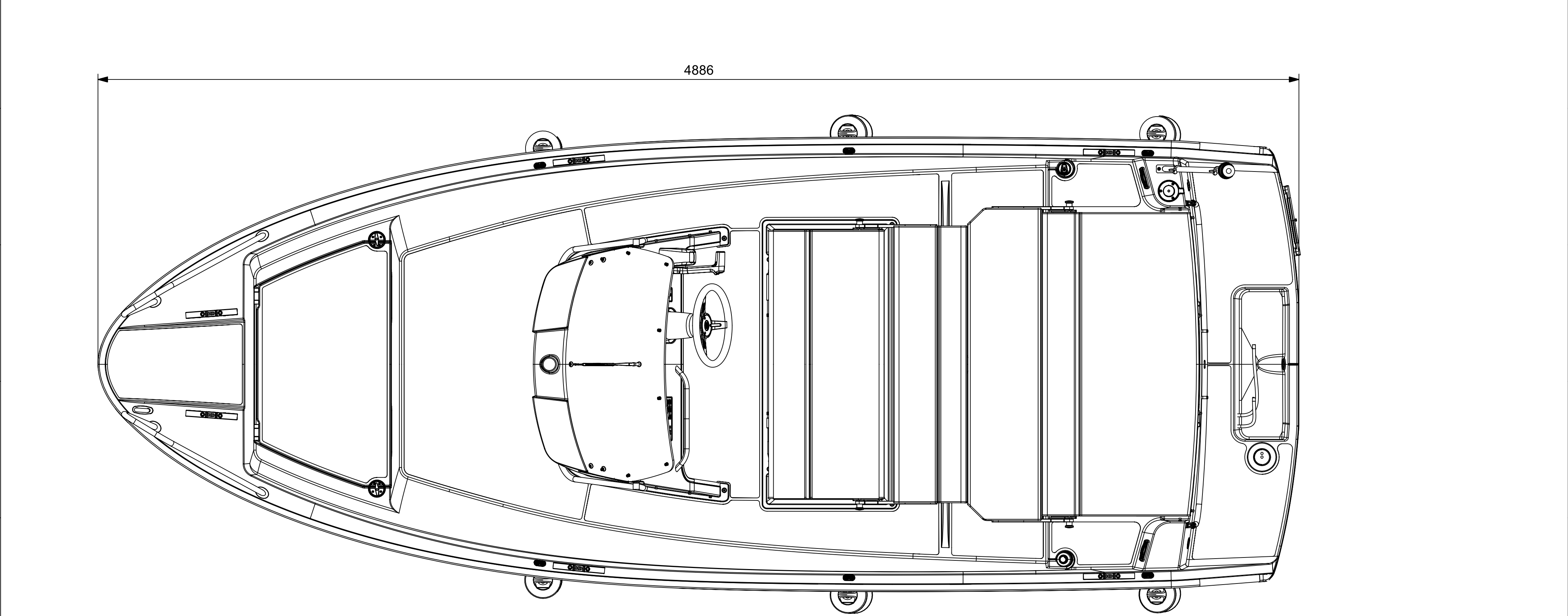
PLAN - excluding engine
